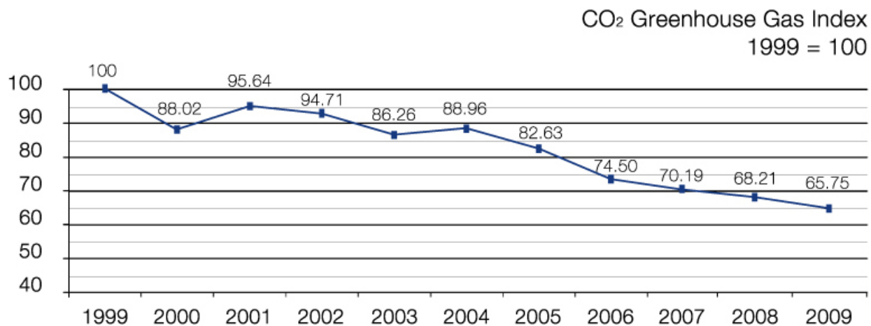
CO 2 Greenhouse Gas
